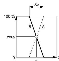
P-controller B03811
