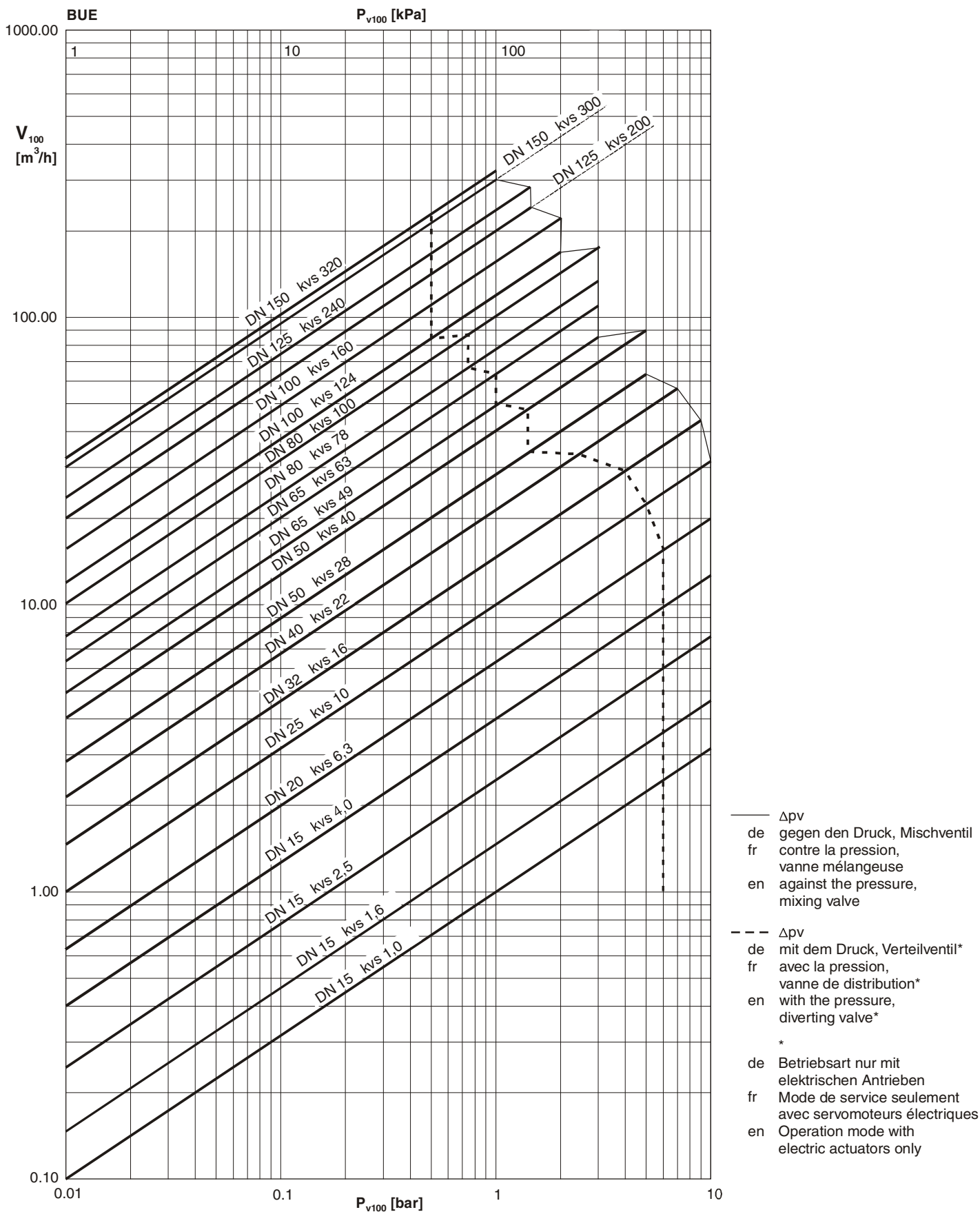
Pressure loss table
